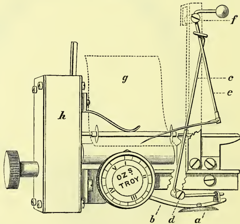
FIG. 43. DIAGRAM OF A SPHYGMOGRAPH (Dudgeon's).
